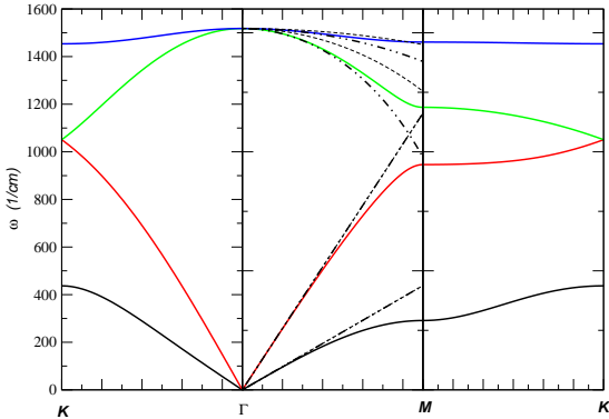
FIG. 1: (color online) Phonon spectrum of the honeycomb lattice, using \alpha = 500 N/m and \beta = 10 N/m, such that the optical frequency at the \Gamma -point is or the order of 1600 \text{ cm}^{-1} . Also shown are the spectra of the simplified model discussed in the text (dashed lines) and the effective model discussed in Appendix A (dashed-dotted lines).
