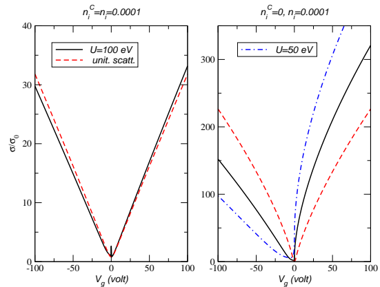
FIG. 7: (color online) Left: Conductivity \sigma(\mu) , in units of \sigma_0 = \pi e^2/(2h) , considering both short range and charged scatterers. Right: Conductivity \sigma(\mu) when the influence of charge scatterers is removed.
