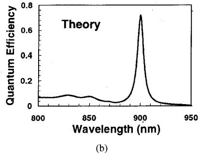
Fig. 2. (a) Measured photoresponse of RCE photodiode and (b) simulated photoresponse of the same structure.
