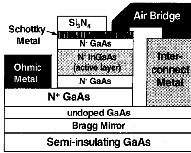
Fig. 1. Diagram showing the cross section of a fabricated RCE Schottky photodiode.
